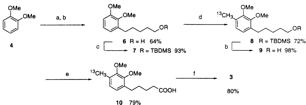
Scheme 1: (a) n -BuLi, THF then I-(CH 2 ) 5 -OTBDMS; (b) TBAF, THF; (c) TBDMSCl, imidazole, DMF; (d) s -BuLi, TMEDA, Et 2 O then [ 13 C]MeI; (e) PDC, DMF; (f) BBr 3 , CH 2 Cl 2 , -78°C.
