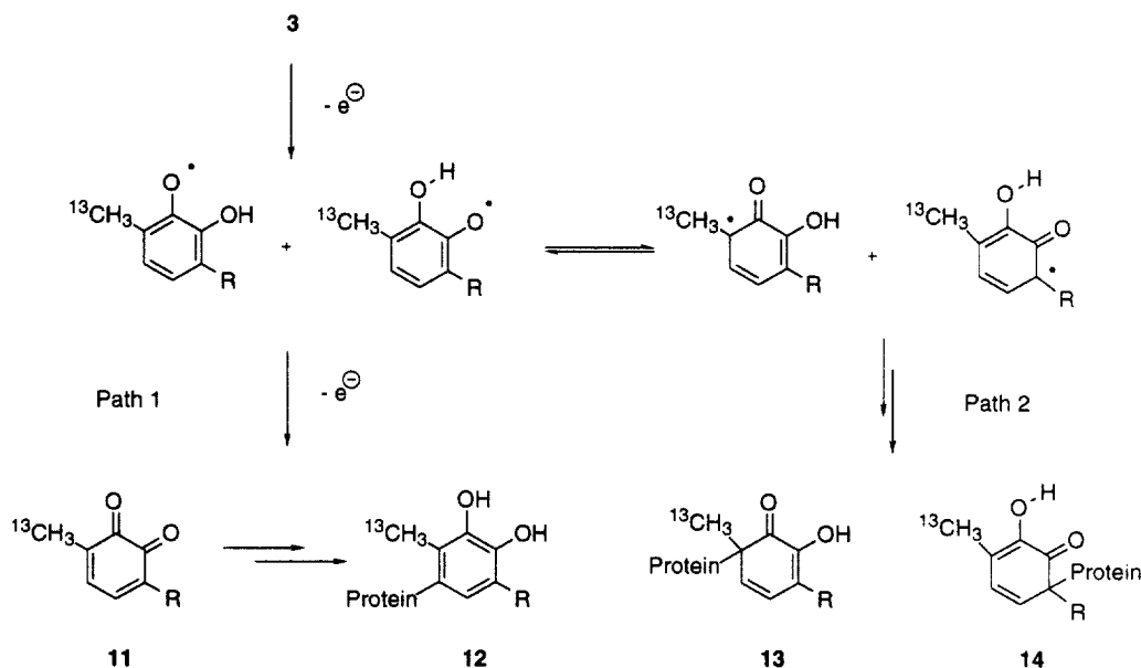
Scheme 2: Possible reaction pathways of 3 with HSA in phosphate buffer at pH 7.4 in the presence of oxygen
