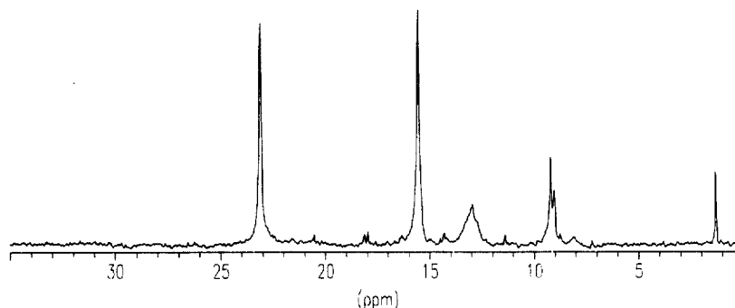
Figure 2: ^{13}\text{C}\{^1\text{H}\} DEPT 135 spectrum of HSA incubated with compound 3 in air in phosphate buffer.
