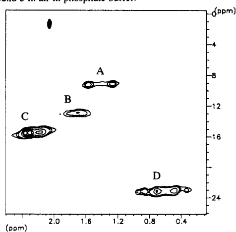
Figure 3: HSQC of HSA incubated with compound 3 in air at pH 7.4 in phosphate buffer.
