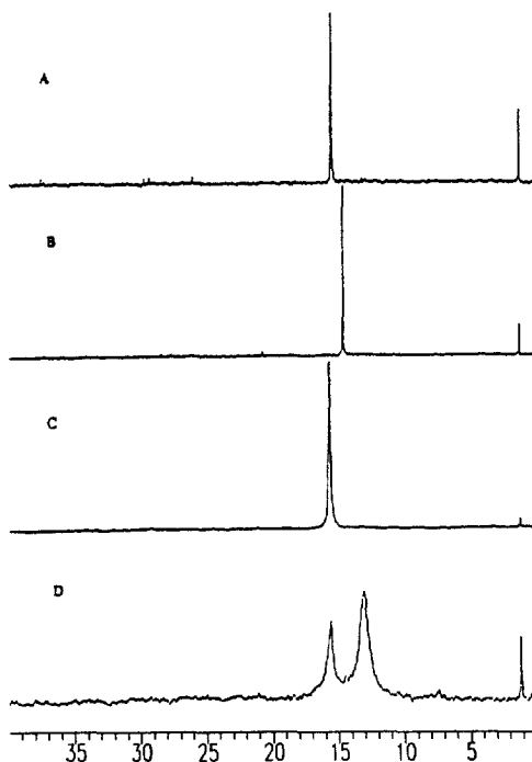
Figure 1: A; 13 C NMR of compound 3 in a 1:1 mixture of phosphate buffer/D 2 O at pH 7.4. B; 13 C NMR of compound 3 oxidized with sodium periodate in a 1:1 mixture of phosphate buffer/D 2 O at pH 7.4. C; 13 C NMR of compound 3 in a 1:1 mixture of phosphate buffer/D 2 O at pH 7.4 in the presence of HSA. D; 13 C NMR of compound 3 oxidized with sodium periodate in a 1:1 mixture of phosphate buffer/D 2 O at pH 7.4 in the presence of HSA.
